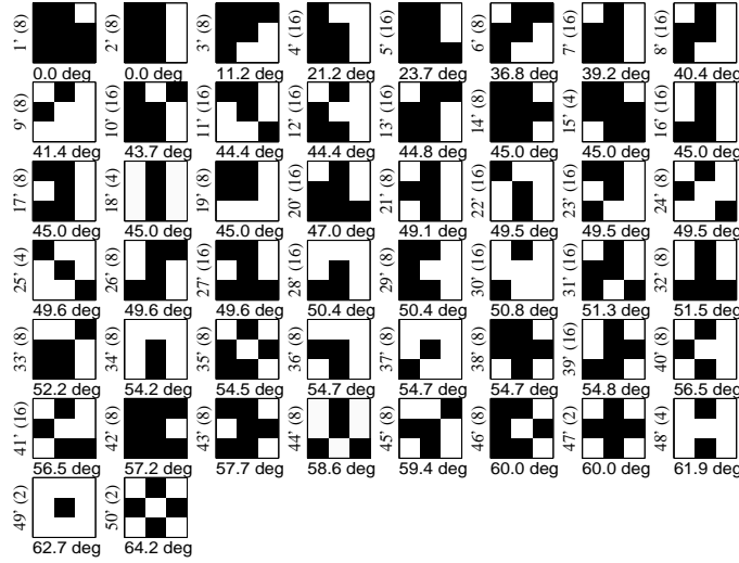
Figure 18. The 50 symmetry classes of binary patches arranged according to increasing \theta -values, where \theta is the angular distance to the closest point on the surface of ideal step edges. The number below each displayed patch represents this distance. The number in parenthesis left of each patch represents the number of binary patches in each equivalence class.
