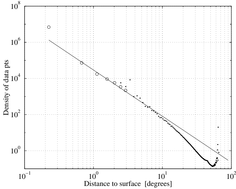
Figure 14. Log-log plot of the average density function p(\theta) for optical data. For \theta < 10 degrees, p(\theta) \sim \theta^{-2.5} (solid line). The circles represent the values of the ratio \frac{N(\theta)/N_{\text{tot}}}{V(\theta)/V_{\text{tot}}} for extrapolated values of V(\theta) when \theta is small (Figure 13b, bottom).
