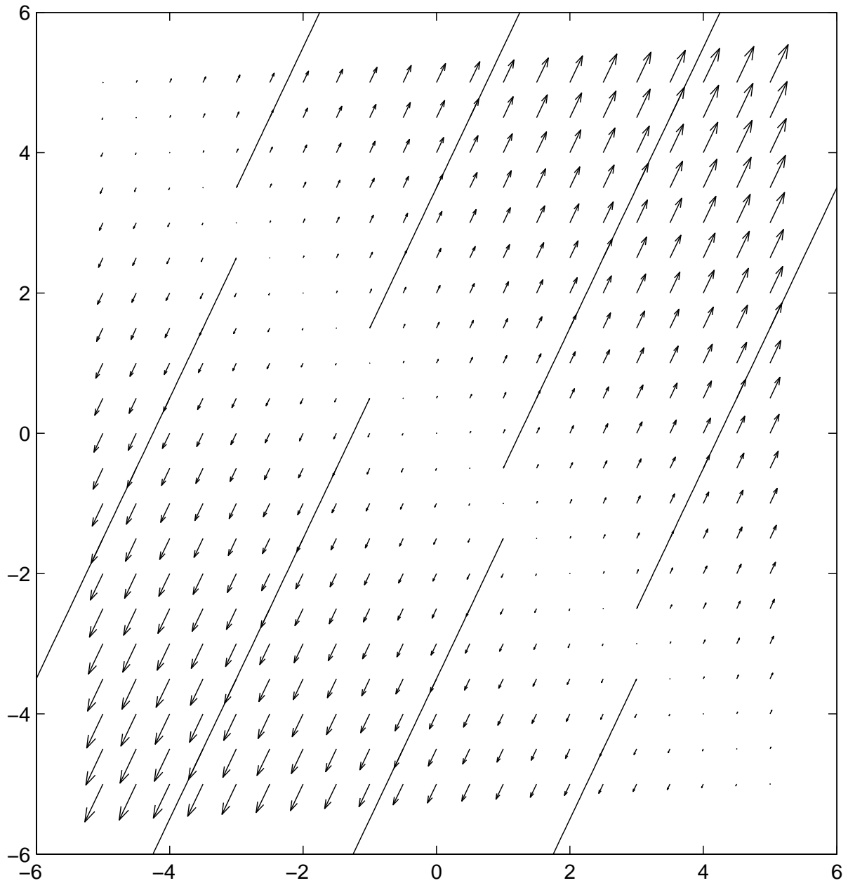
Figure 1: Direction field and sample trajectories for linear system with (a, b, c, d) = (1, 1, 2, 2) .
