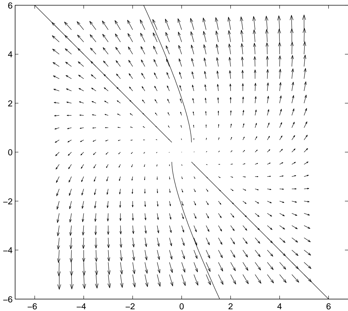
Figure 1: Direction field and sample trajectories for linear system with (a, b, c, d) = (1, -1, 1, 3) .
