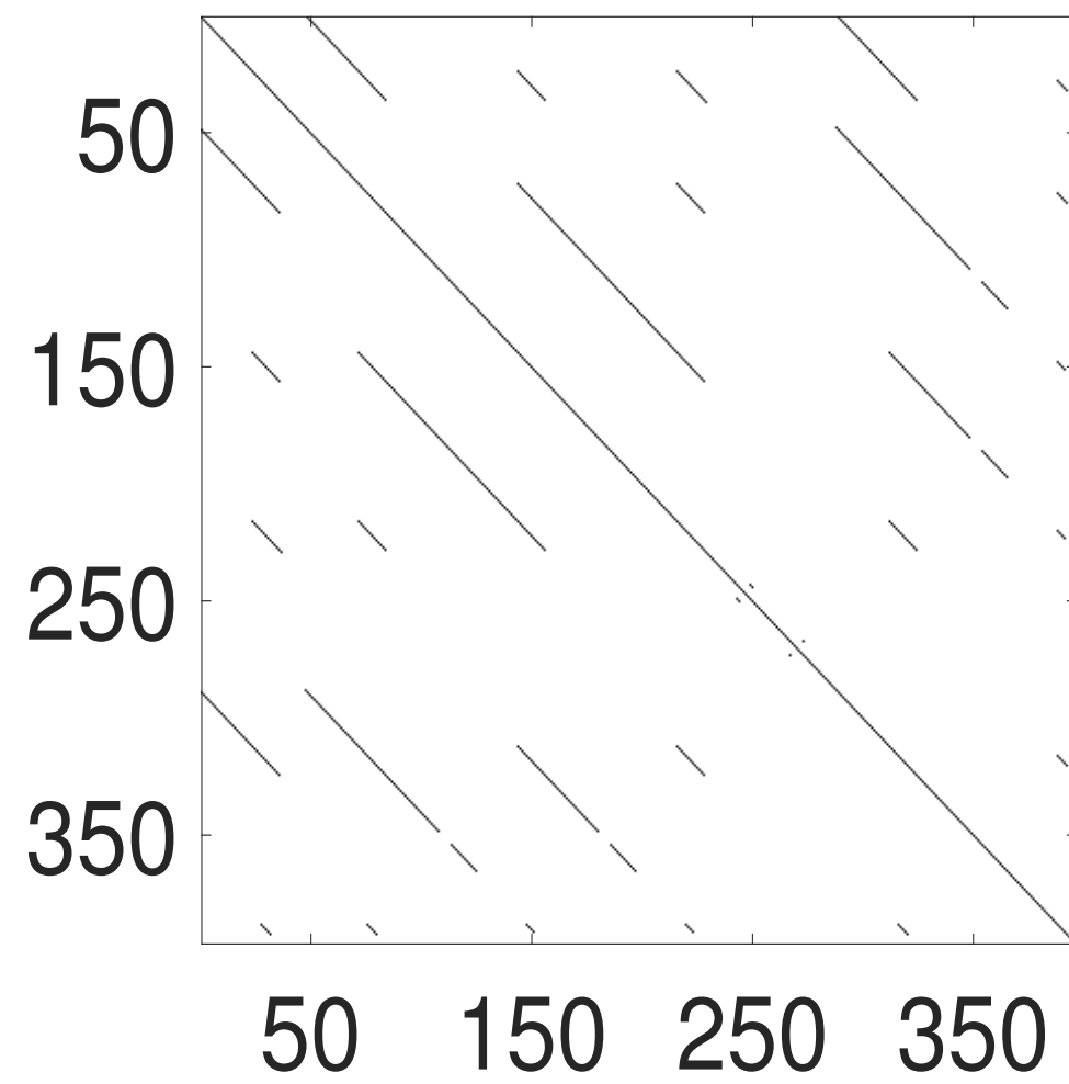
Figure 1: Thresholded SDM
