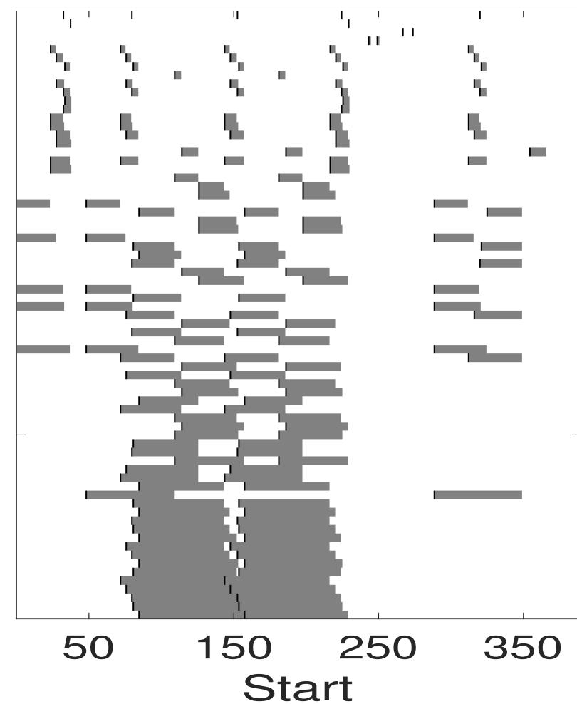
Figure 2: Aligned Hierarchies
