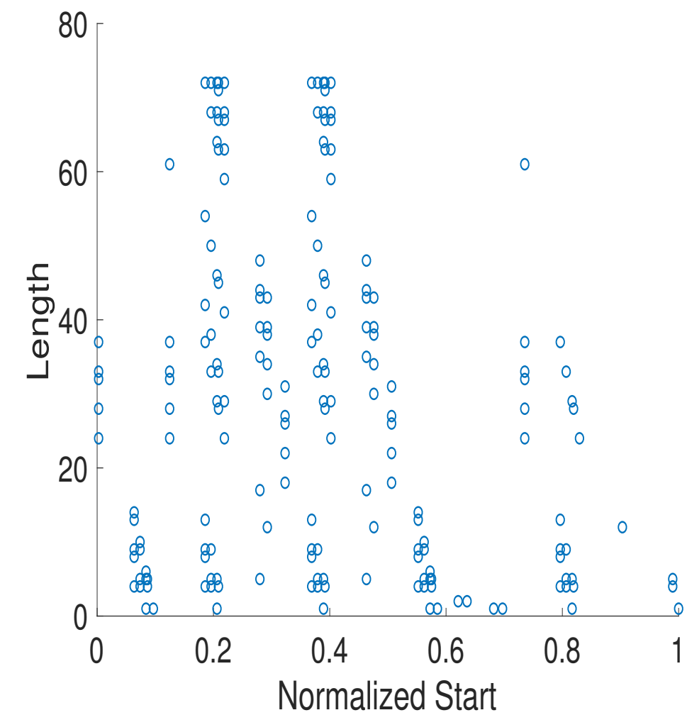
Figure 4: S_{NL} diagram ( \alpha = 1 )
