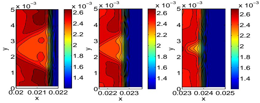
Figure 30: Density results of Example 5.1: WENO5/SR with 200 \times 40 , CFL=0.1 and N_r = 2 at t = 1.5 \times 10^{-7} , t = 1.6 \times 10^{-7} and t = 1.7 \times 10^{-7} .
