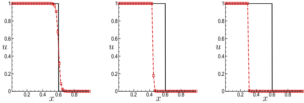
Figure 2: Results of Example 2.2 by the splitting WENO5 scheme with N = 50 at t = 0.3 . Solid line: exact solution; dashed line with symbols: computed solution. Left: \mu = 10 , CFL=0.5; middle: \mu = 800 , CFL=0.1; right: \mu = 10000 , CFL=0.05.
