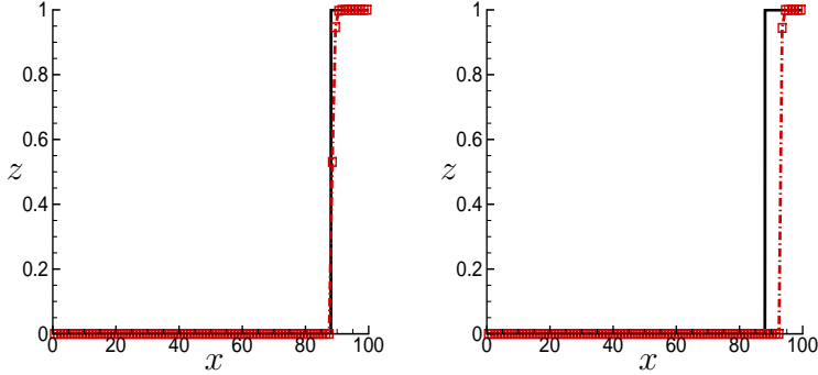
Figure 23: Computed mass fraction for the Heaviside Example 4.4 at t = 8 . Solid line: reference solution. Dashed line with symbols: numerical solution. Left: WENO5/SR with N = 100 , CFL=0.1; right: splitting WENO5 with N = 100 , CFL=0.1.
