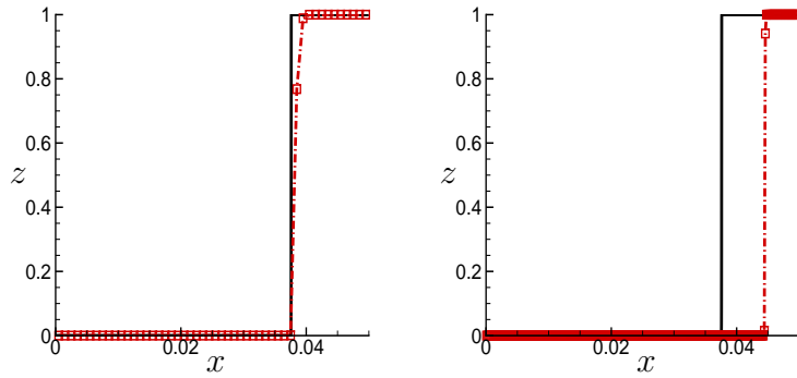
Figure 14: Computed mass fraction for the Heaviside Example 4.2 at t = 3 \times 10^{-7} . Solid line: reference solution. Dashed line with symbols: numerical solution. Left: WENO5/SR with N = 50 , \text{CFL}=0.1 , N_r = 10 ; right: splitting WENO5 with N = 300 , \text{CFL}=0.01 .
