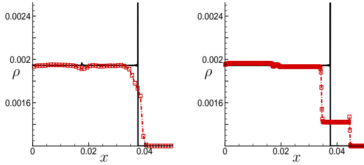
Figure 13: Computed density for the Heaviside Example 4.2 at t = 3 \times 10^{-7} . Solid line: reference solution. Dashed line with symbols: numerical solution. Left: WENO5/SR with N = 50 , \text{CFL}=0.1 , N_r = 10 ; right: splitting WENO5 with N = 300 , \text{CFL}=0.01 .
