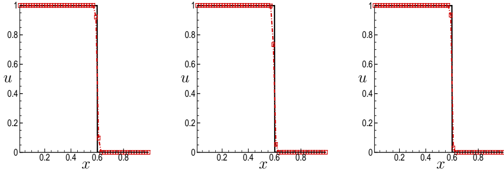
Figure 1: Results of Example 2.2 by the anti-diffusive WENO5/SR with N = 50 at t = 0.3 . Solid line: exact solution; dashed line with symbols: computed solution. Left: \mu = 10 , CFL=0.5; middle: \mu = 800 , CFL=0.5; right: \mu = 10000 , CFL=0.2.
