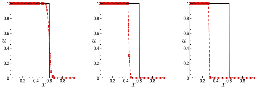
Figure 3: Results of Example 2.2 by the standard WENO5 without splitting scheme with N = 50 at t = 0.3 . Solid line: exact solution; dashed line with symbols: computed solution. Left: \mu = 10 , CFL=0.5; middle: \mu = 800 , CFL=0.1; right: \mu = 10000 , CFL=0.02.
