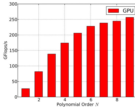
Fig. 1.10 Floating point performance in GFlops/s achieved by our auto-tuning solver on a large 3D Maxwell problem in single precision on an Nvidia GTX 280. Performance is calculated by measuring wall time from one time step to the next and dividing the number of flops performed (including timestepping) by this value.
