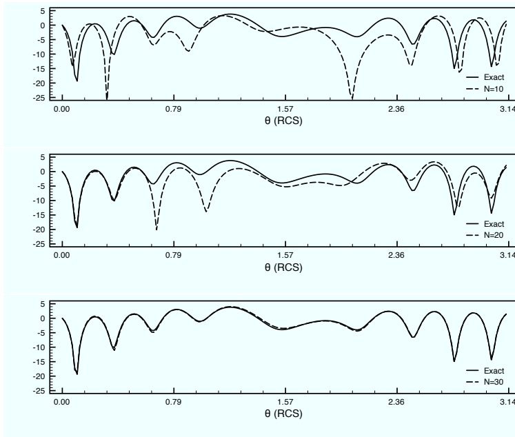
FIGURE 15. Exact and approximated RCS-signal by the Reduced Basis Method for test case iii) with k = 23.8 and for three different dimensions of the reduced basis.
