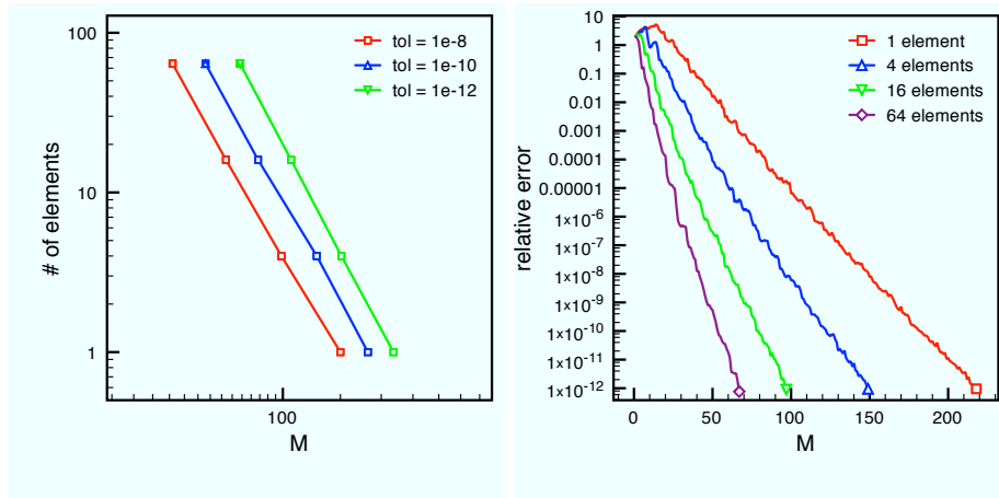
FIGURE 9. The length of the EEIM expansion M versus the number of elements needed for test case iv) and three different error tolerances (left). Accuracy of the EEIM with respect of the length of the EEIM expansion M for different numbers of resulting elements (right).
