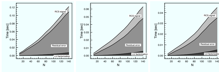
FIGURE 14. The time of the subtasks of the online procedure of three different versions of the Reduced Basis Method for different dimensions of the Reduced Basis. The time (measured in seconds) corresponds to the average computing time of the RCS-signal for a parameter value for the test example iv).
