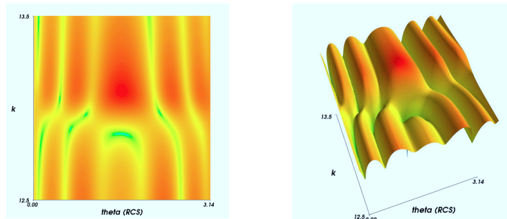
FIGURE 18. Two different plots of a zoom of the RCS-signal in function of the wave number k \in [12.5, 13.5] for test case iii).
