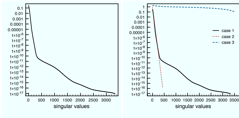
FIGURE 1. Singular value decomposition of the matrix consisting of column-wise Boundary Element solutions for different parameters values of a real case (a). Different types of SVD-profiles (b).
