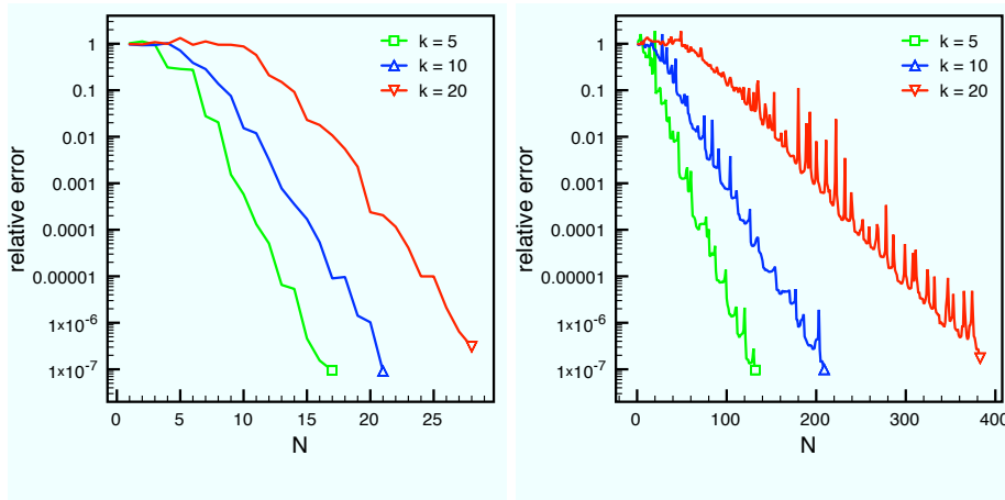
FIGURE 11. Accuracy of the Reduced Basis Method for test case i) (left) and ii) (right) for different values of the wave number k .
