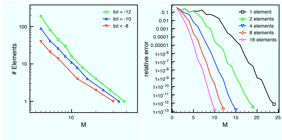
FIGURE 8. The length of the EEIM expansion M versus the number of elements needed for test case i) and three different error tolerances (left). Accuracy of the EEIM with respect of the length of the EEIM expansion M for different numbers of resulting elements (right).
