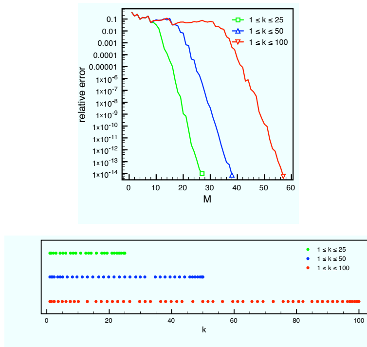
FIGURE 4. Relative error in the test case i) for different values of k_{\max} depending on the length M of the expansion (top) and the corresponding picked parameter values (bottom).
