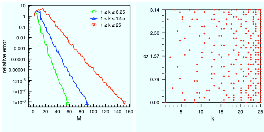
FIGURE 7. Relative error in the test case iv) for different values of k_{max} depending on the length M of the expansion (left) and the corresponding picked parameter values for k = 25 (right).
