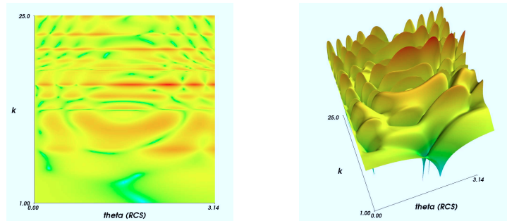
FIGURE 17. Two different plots of the RCS-signal in function of the wave number k \in [1, 25] for test case iii).
