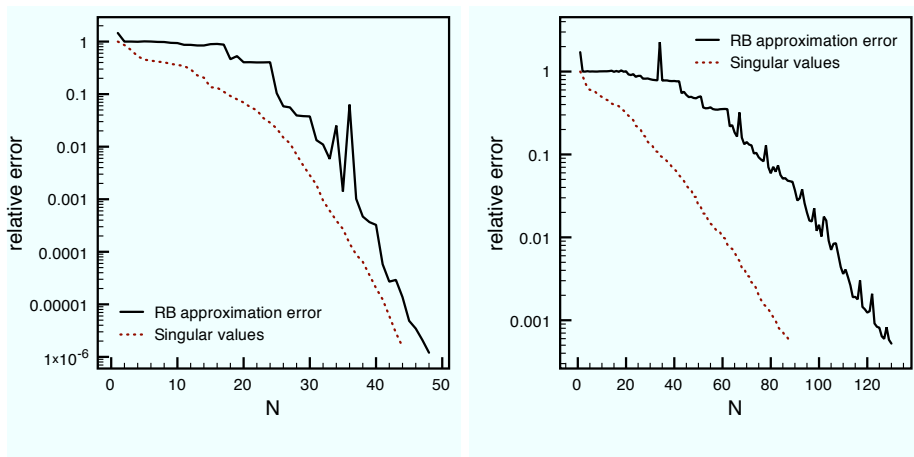
FIGURE 12. Accuracy of the Reduced Basis Method for test case iii) (left) and iv) (right) and comparison to the optimal accuracy given by the singular values.
