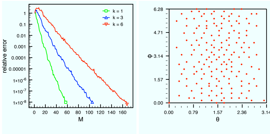
FIGURE 6. Relative error in the test case iii) for different values of k depending on the length M of the expansion (left) and the corresponding picked parameter values for k = 6 (right).
