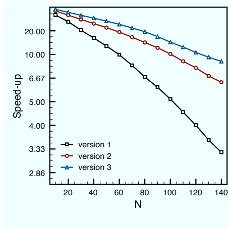
FIGURE 13. Speed-up for three different versions of the online procedure of the Reduced Basis Method with respect to the computing time using the Boundary Element Method in function of the dimension of the Reduced basis. Test example iv) is considered.
