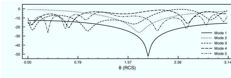
FIGURE 16. Unnormalized RCS-signal corresponding to the first five reduced basis functions for test case iii).
