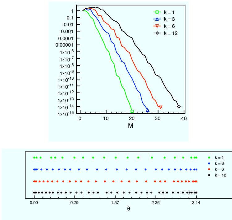
FIGURE 5. Relative error in the test case ii) for different values of k depending on the length M of the expansion (top) and the corresponding picked parameter values (bottom).
