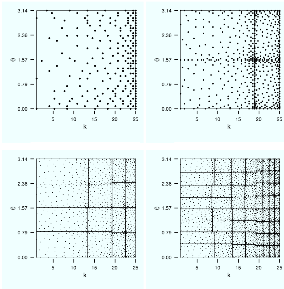
FIGURE 10. Picked parameter values and subdivision of the parameter domain for different levels of refinements. The empirical interpolation satisfies a relative error tolerance of 10^{-12} for all four cases but with different lengths of the series per element, i.e. M = 218, 151, 106, 74 .
