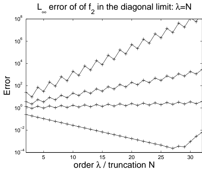
Figure 1: Log of maximum pointwise errors of the sequences \mathcal{E}(1, N) = E(N, N) for the function f_2(x; z) = 1/\log(z^2 + x^2 + 1) for different values of z and \beta = 1 . As z decreases, the pole moves closer to the real axis and causes divergence of the sequence of approximants.
