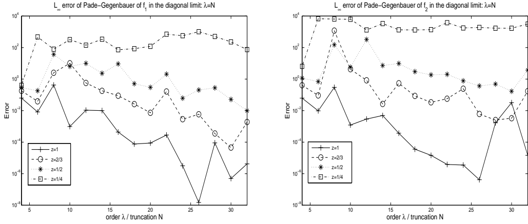
Figure 3: Log of maximum pointwise error of sequences of Padé-Gegenbauer interpolants of the function for various values of z and fixed M = N/2, L = N/2 with \beta = 1 . Left: f_1 Right: f_2 .
