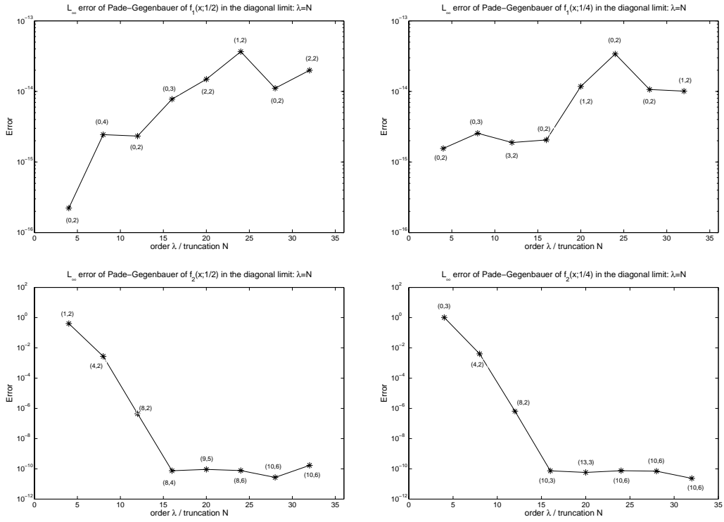
Figure 4: L_\infty error of sequences of Padé-Gegenbauer interpolants for various values of z of both functions and \beta = 1 . The interpolant of order (M, L) that minimizes the L_\infty error is shown on the plot. Top: f_1(x; 1/2) and f_1(x; 1/4) Bottom: f_2(x; 1/2) and f_2(x; 1/4)
