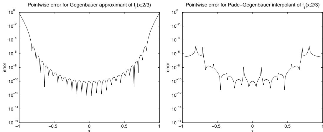
Figure 2: On the left we have the pointwise error of the Gegenbauer approximant of order N = 24 to the function f_1(x; 2/3) . The large error in the narrow region near the boundaries is the Runge phenomenon. The right figure shows the Padé-Gegenbauer interpolant of order (12,12) for the same function and shows the suppression of the Runge phenomenon. Both figures are shown on a uniform grid of 200 points.
