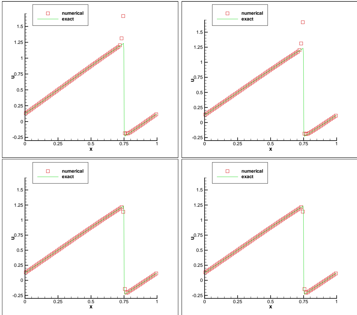
Figure 5.1: Solutions of Burgers equation at time T = 0.5 . Uniform mesh with 80 cells. Top: no limiters; Bottom: with the TVB limiter, M = 40 . Left: P^2 approximation space; Right: E^2(1) approximation space. Solid line: the exact solution; Symbols: numerical solutions (one point per cell).
