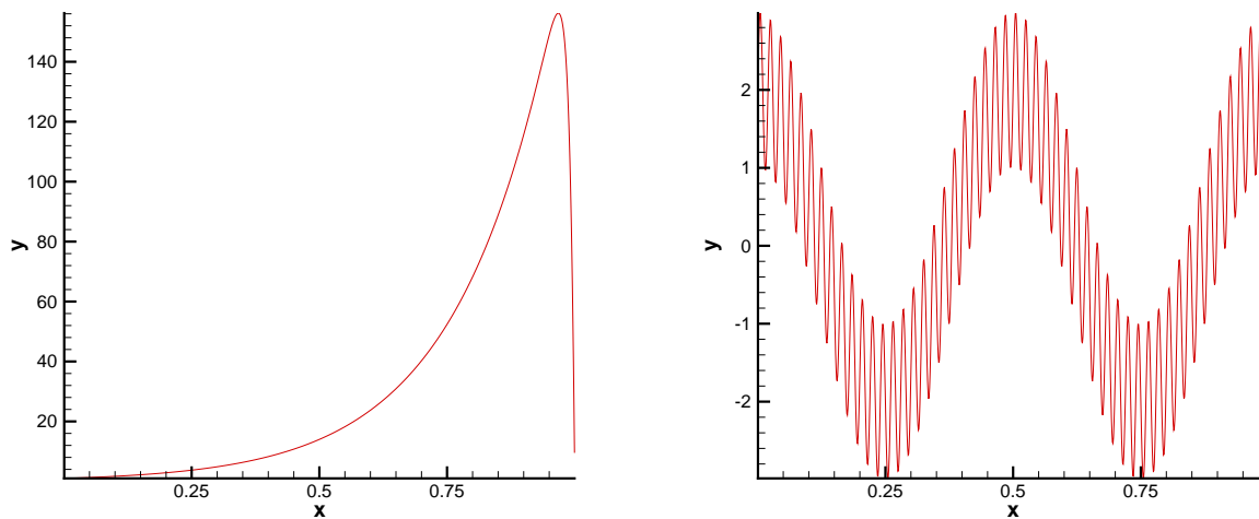
Figure 1.1: Examples of solutions to the boundary layer problem (left) and the highly oscillatory problem (right).
