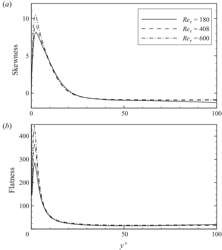
FIGURE 6. Acceleration (a) skewness and (b) flatness factors for three different Re_\tau .
