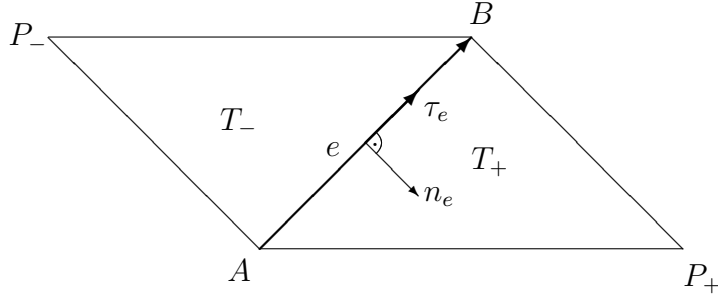
FIGURE 2.1. Two neighboring triangles T_- and T_+ that share the edge e = \partial T_- \cap \partial T_+ with initial node A and end node B and unit normal n_e . The orientation of n_e = n_- = -n_+ equals the outer normal of T_- , and hence, points into T_+ .
