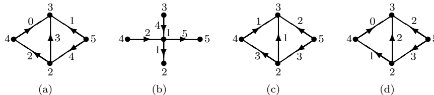
FIGURE 2. Conservative 1-flows and firings
