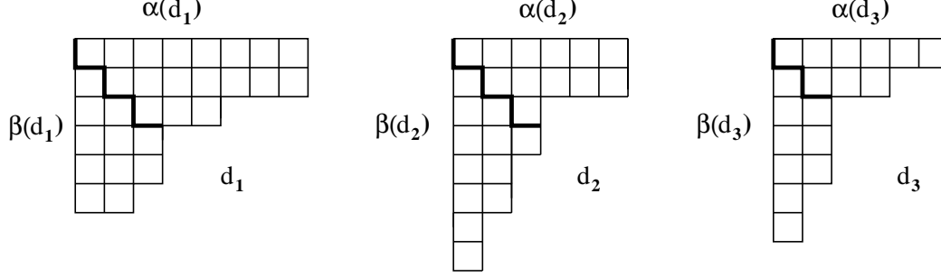
FIGURE 1. Cutting partitions into shifted shapes.
