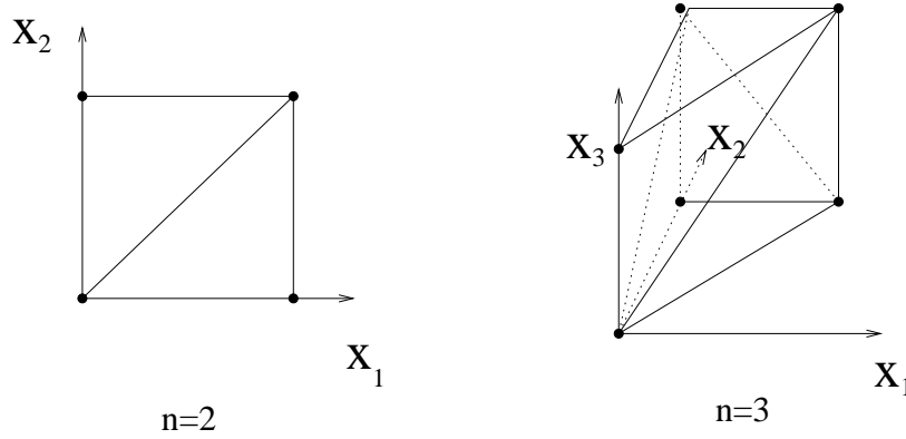
FIGURE 2. A well-known triangulation of a prism over a simplex.
